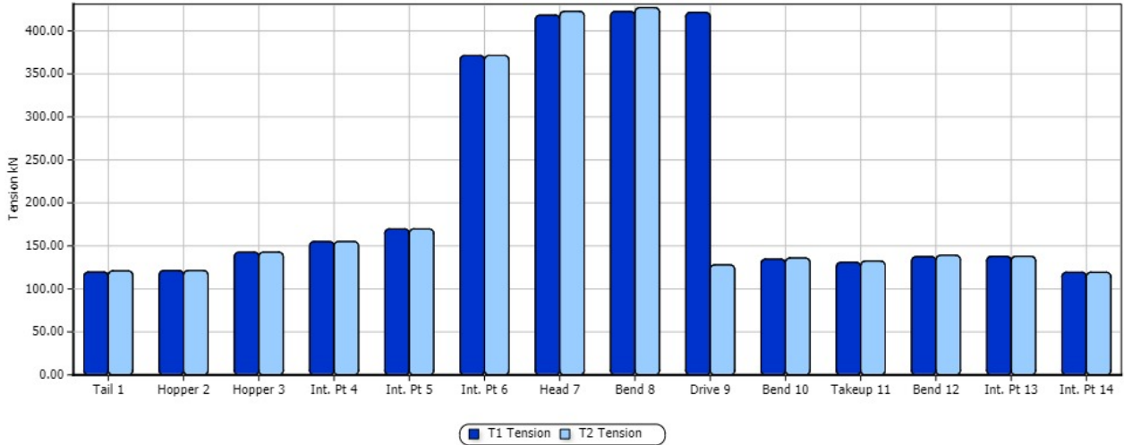
Belt Tensions Run Inclines Loaded Conveyor No. C223
